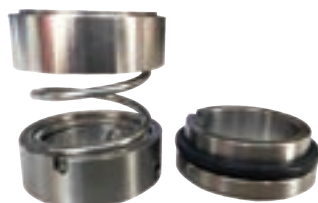
108U Mechanical Seal
